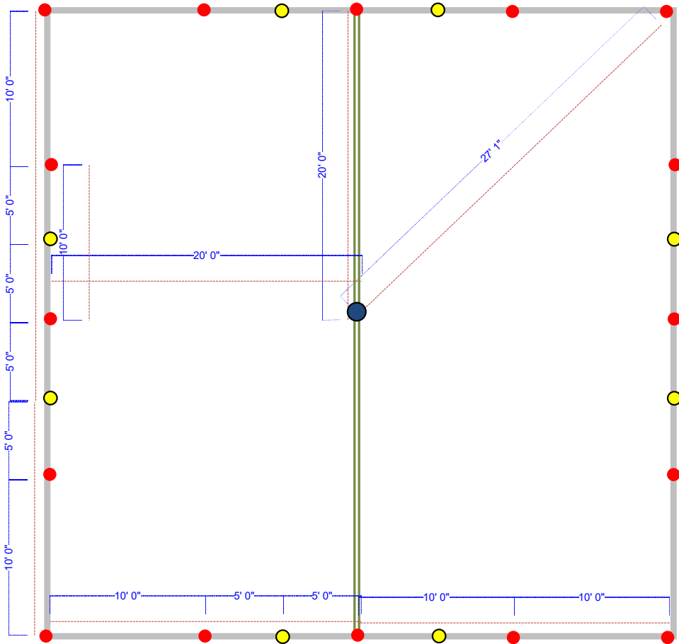
40' x 40' Pole Tent Standard & Wind - Pole Placements
